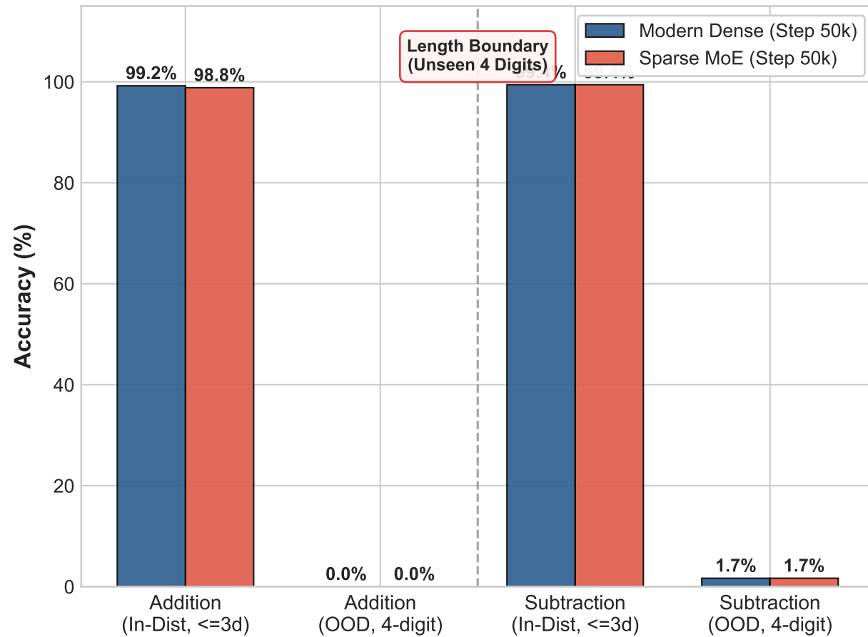
(a) Length Generalization Collapse (4-Digit OOD)
