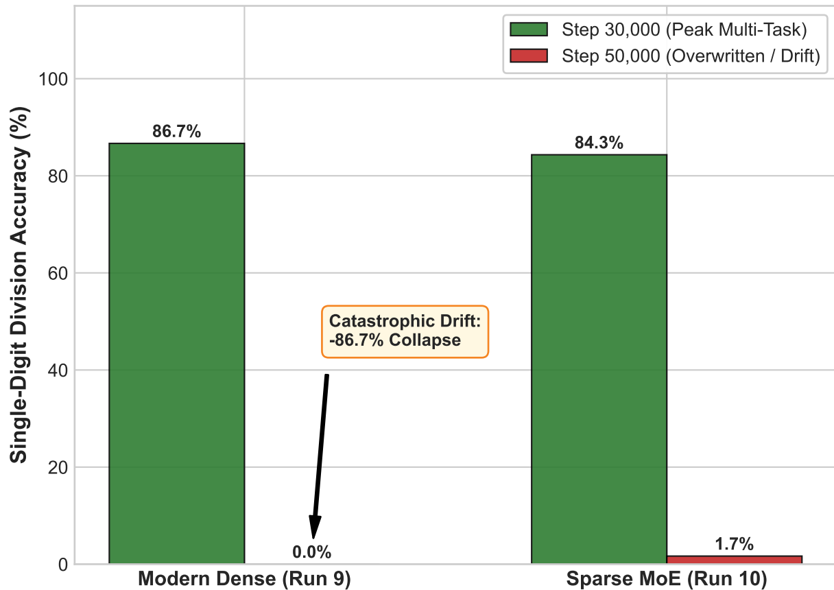
(b) Catastrophic Drift on Single-Digit Division
