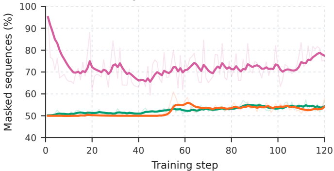
Qwen3.5-9B Math
