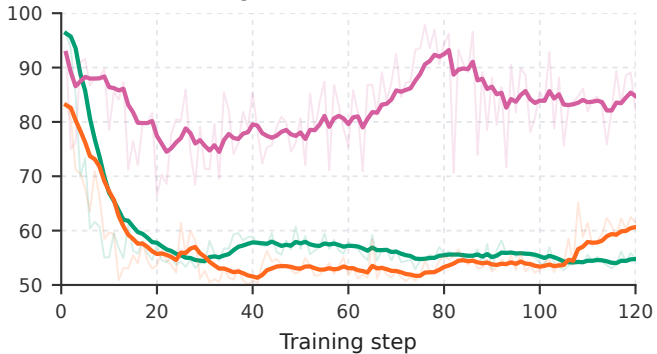
Qwen3.5-9B Code
