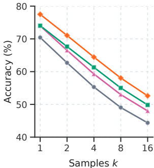
Worst-of- k
