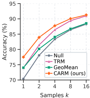
Best-of- k
