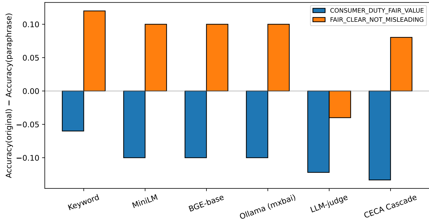
Paraphrase robustness gap (smaller is better)
