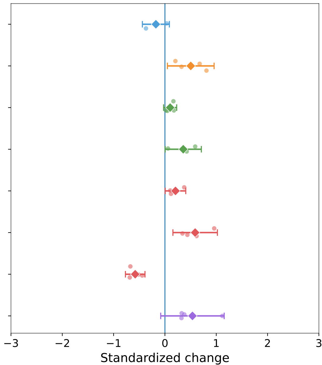
Temperature 0.2→1.0
