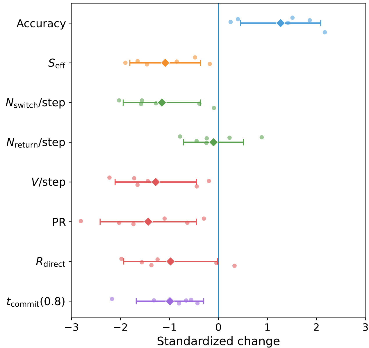
Instruction tuning
