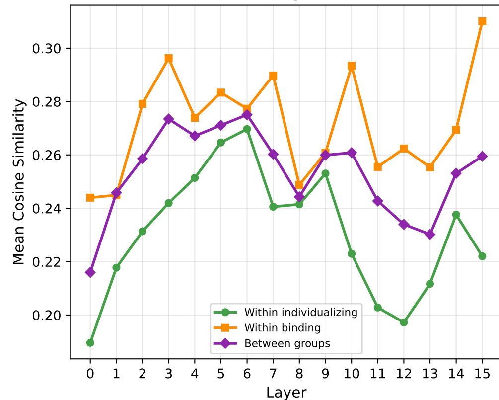
(c) MFT Group Structure
