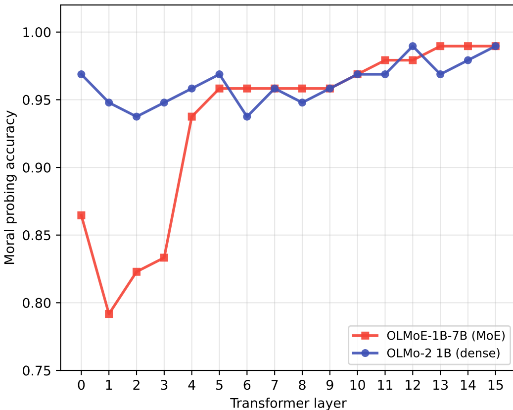
(a) probing accuracy: indistinguishable (peak 99.0%)
