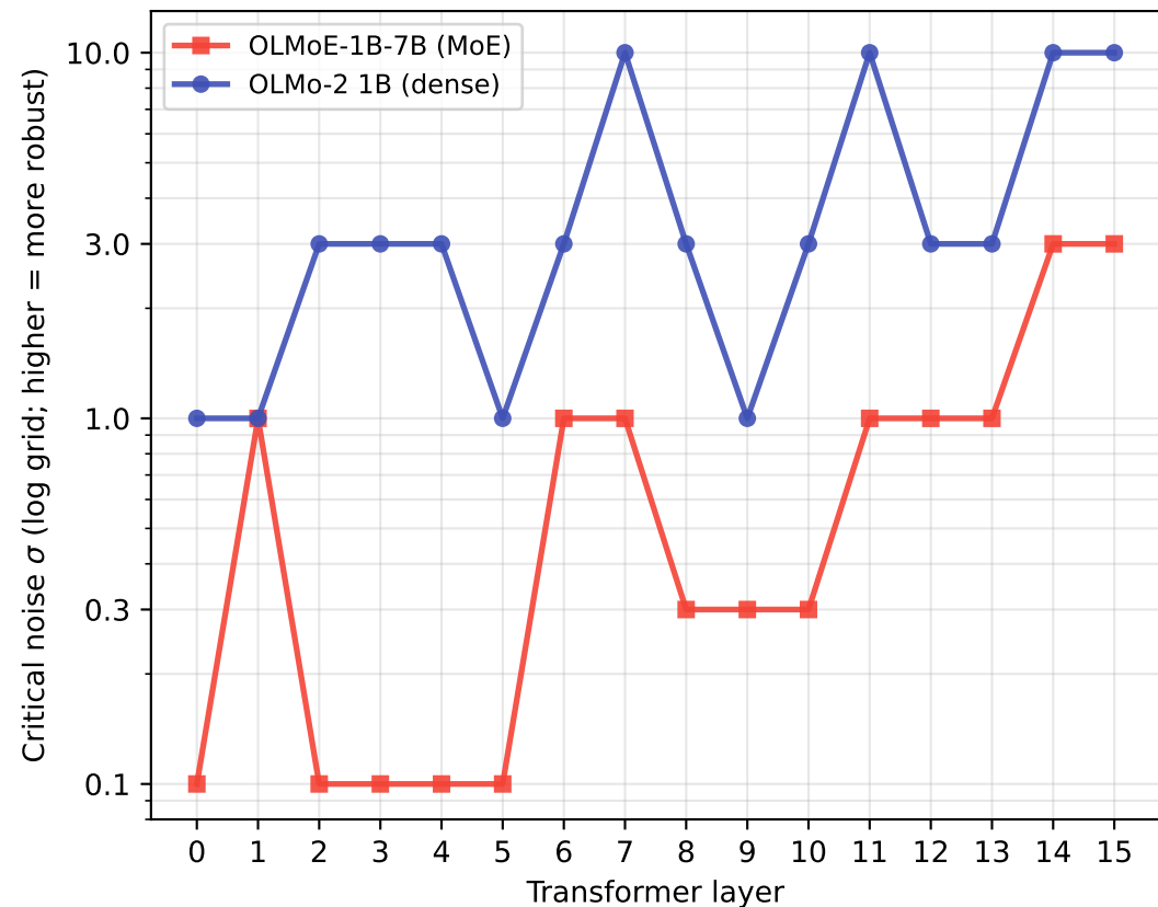
(b) fragility: MoE 5.1× more fragile ( \sigma^* 0.84 vs. 4.25)
