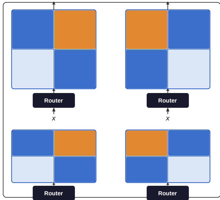
Cell-Wise LoRA-MoE (Decentralized Micro-Routing)
