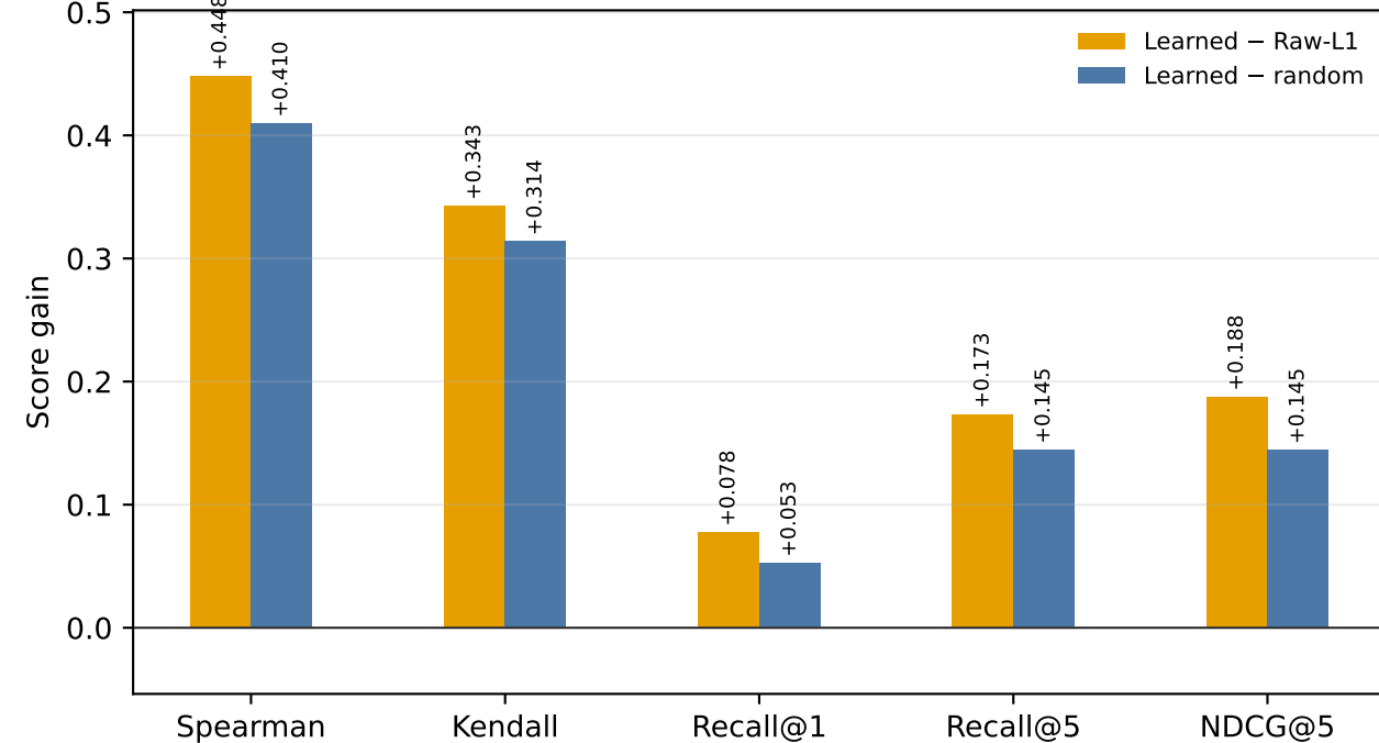
Absolute gain over matched selectors
