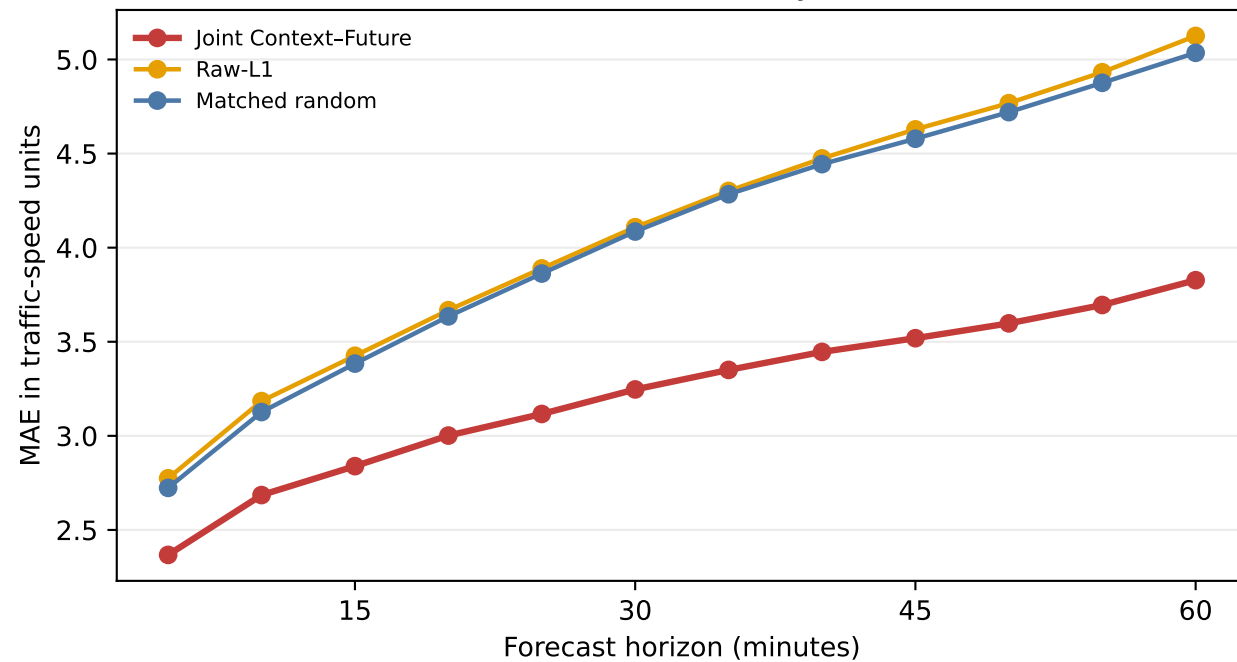
Horizon-wise Memory MAE
