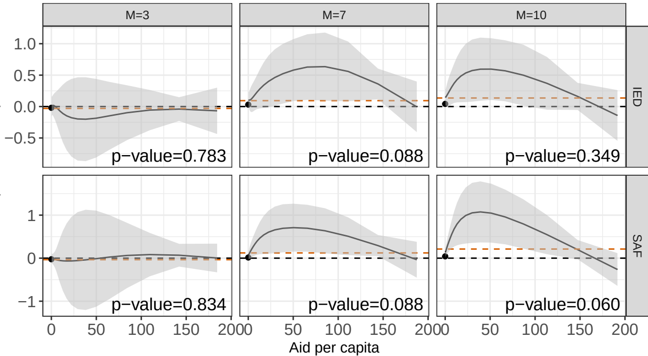
CATE (District Effect)
