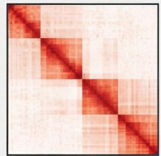
Hi-C Contact Matrix
