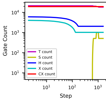
512-bit Adder
