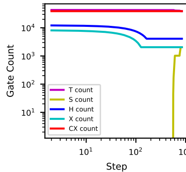
1024-bit Adder
