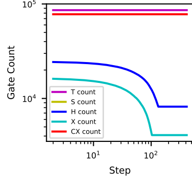
2048-bit Adder
