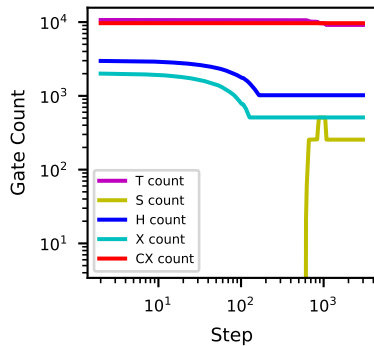
256-bit Adder
