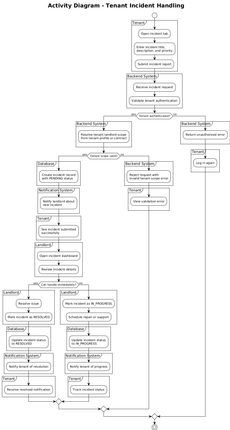
Figure 4.6: Activity Diagram - Tenant Incident Handling
