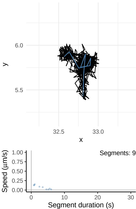
Perinuclear Lysosome Path 2
