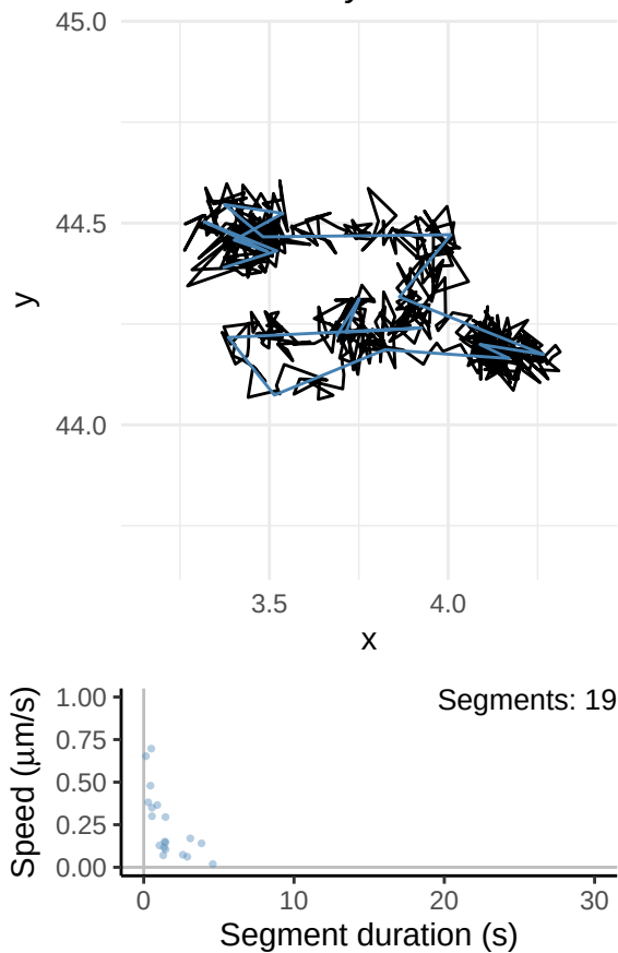
Perinuclear Lysosome Path 1
