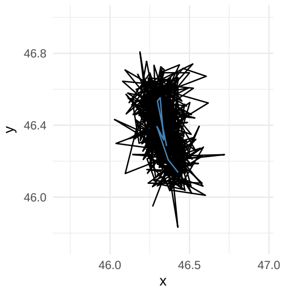
Perinuclear Lysosome Path 3
