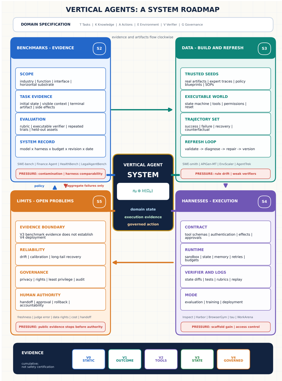
Figure 2: A system roadmap for vertical agents. The center couples a model policy with its domain execution harness. The four surrounding panels organize benchmarks, data synthesis, harnesses, and evidence boundaries; the upper band records the six domain-specific objects, while the lower V0–V4 ladder records cumulative public evidence rather than a safety certification.
