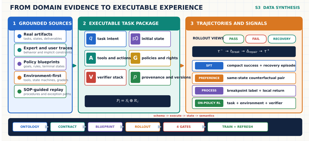
Figure 3: From domain evidence to executable experience. Grounded sources are packaged with initial state, tools, policies, verifiers, and provenance. Failure-aware rollout records preserve breakpoints, minimal repairs, and counterfactual contrasts, then route them to objective-specific learning signals. The footer shows the six-stage construction and refresh loop.
