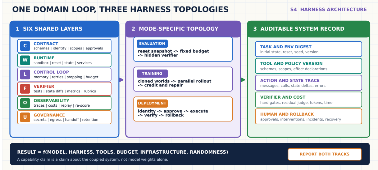
Figure 4: One domain loop, three harness topologies. A complete harness shares six layers across evaluation, training, and deployment, but each mode instantiates a different control topology. An auditable system record is required to separate model gains from harness, tool, budget, infrastructure, and stochastic effects.
