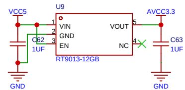
VCC5转AVCC3.3
