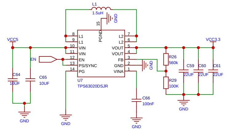
VCC5转VCC3.3
