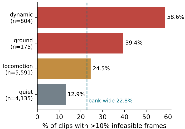
(a) by motion category
