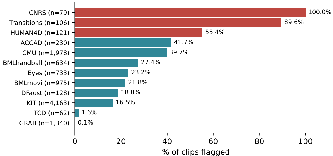
(b) by source dataset — 0.1% → 100% under ONE retargeting pipeline
