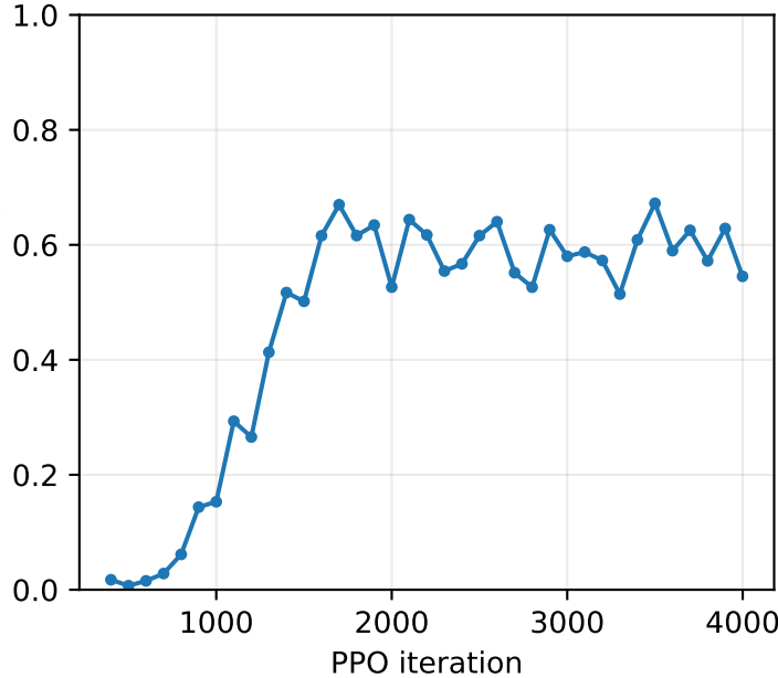
Seed 12 sampler diagnostic — exploratory; no policy-benefit test
