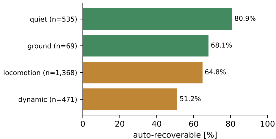
(b) by category — ballistics correctly resist repair
