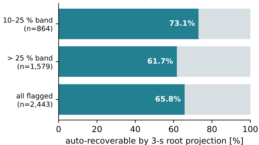
(a) by severity
