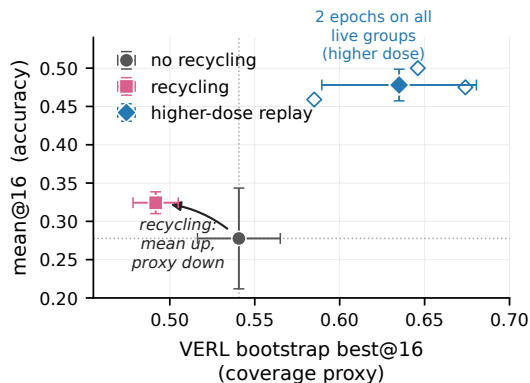
Figure 7: Secondary Countdown accuracy–coverage-proxy record. Error bars are sample standard deviations across three seeds; seed 3 for B1/B2 is aggregate-only. The recycling-package aggregate has higher mean@16 and lower VERL bootstrap best@16. The live-group replay control uses two optimizer epochs on every live group, so it cannot separate dose from update direction.
