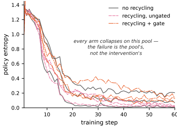
Figure 11: Jugs pool-conditionality: every arm collapses ( 3 \text{ arms} \times 3 \text{ seeds} ). On a pool whose learnable band is a single stratum of 1–2-move template solutions, plain MaxRL’s policy entropy collapses ( 1.36 \rightarrow 0.01\text{--}0.21 ) with no recycling involved; ungated recycling ends lowest, and the gate merely delays the fall. Rollout-set diversity at initialization is the design gate this suite motivates (§9).
