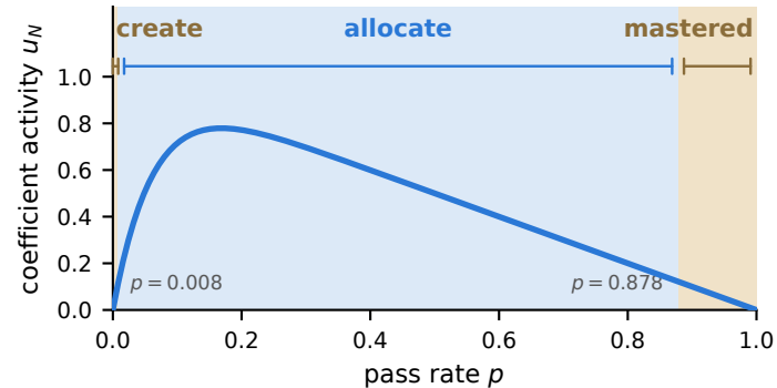
A where a sampler can act ( N = 16, B = 8 )
