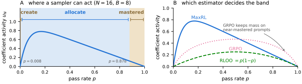
Figure 1: The three-regime map: the teacher allocates, hindsight creates, the estimator decides whether either is safe. (A) Coefficient activity has exact zeros at p=0 and p=1 , so the pass-rate axis splits into a band where a sampler can redistribute existing signal and two regions where no priority rule can help. Edges are budget-dependent: with B groups per step a task is operationally dead at budget when it yields under one live group, B\{1 - (1 - p)^N\} < 1 ; drawn at B=8 , N=16 . Relabeling is the only channel that adds signal outside the band (App. C). (B) Which estimator is deployed decides the band’s shape. GRPO’s geometry retains mass on near-mastered prompts, so a frontier curriculum is not automatically safe under it.
