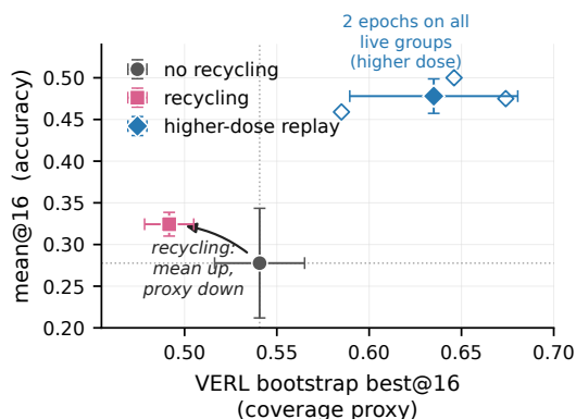
Figure 6: Secondary Countdown accuracy–coverage-proxy record. Error bars are sample standard deviations across three seeds; seed 3 for B1/B2 is aggregate-only. The recycling-package aggregate has higher mean@16 and lower VERL bootstrap best@16. The live-group replay control uses two optimizer epochs on every live group, so it cannot separate dose from update direction.
