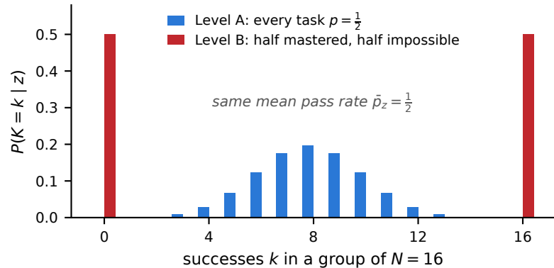
A two units, one mean, two count laws
