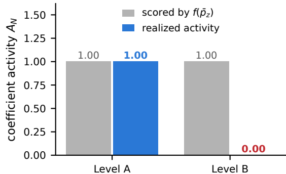
B what the estimator actually emits
