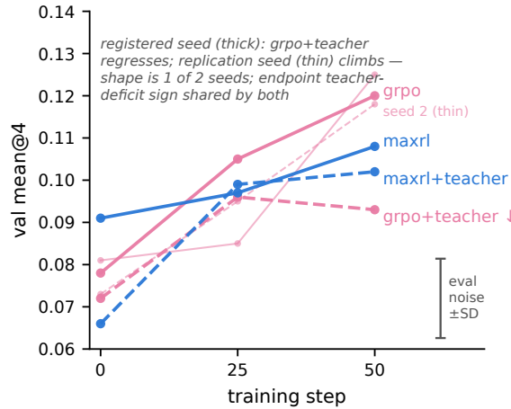
Figure 6: GSM8K 2 \times 2 (pre-registered; both GRPO seeds shown as paired trajectories — registered seed thick, replication seed thin; the gray bar is the repeated-eval noise floor of one fixed checkpoint, \pm SD .0094 , drawn once as a scale, not per-point method uncertainty). On the registered run GRPO+teacher is the only cell that regresses in its second half (P-G2; the load-bearing statistic is the endpoint gap vs. plain GRPO, 2\text{--}4\times the repeated-eval noise — a descriptive signal-to-noise read, not a test); the replication seed, with weaker measured steering, climbs instead — the regression shape is 1 of 2 seeds, while the endpoint teacher-deficit sign holds in both (§6.7); under MaxRL the identical teacher trains stably to its best value but does not beat uniform at this budget (P-G1: null).
