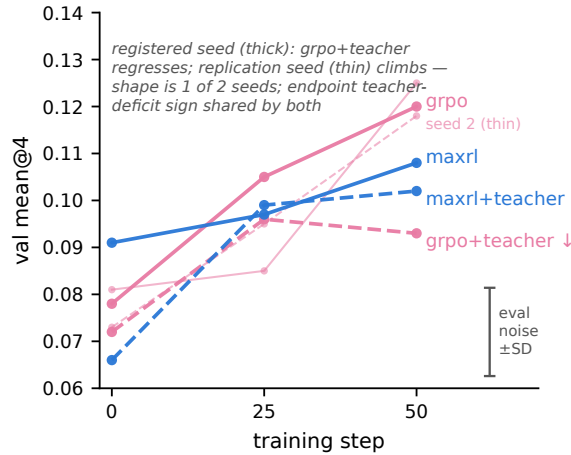
Figure 6: GSM8K 2×2, val mean@4 over training. Both GRPO seeds shown as paired trajectories (registered seed thick, replication thin); gray bar: repeated-eval noise floor of one fixed checkpoint ( \pm SD .0094), drawn once as a scale. On the registered run GRPO+teacher is the only cell that regresses in its second half; the replication seed climbs instead. §6.7 gives the statistics and the steering telemetry that separates the two seeds.
