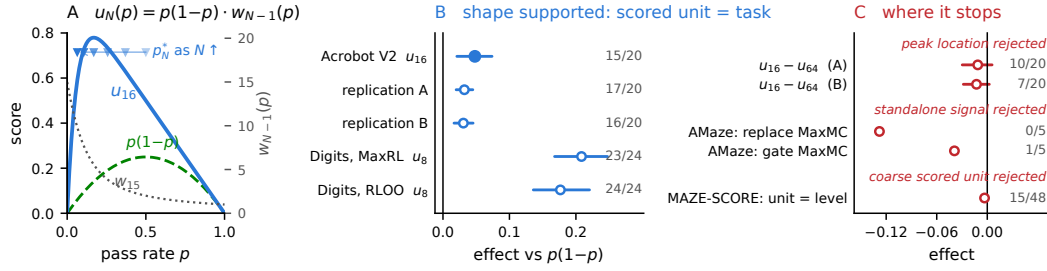
Figure 1: One identity and one claim boundary. (A) Activity is learnability reweighted by MaxRL’s own objective weight (Cor. 1); the peak is derived, not tuned. (B) Every measured shape contrast against the N=2 slice, in studies whose scored unit is the i.i.d. unit; paired-bootstrap 95% intervals, positive-pair counts, filled marker for the one frozen primary. (C) The three preregistered boundaries, the last being the one study scoring a strict aggregate (Cor. 2). Panel-C rows are different endpoints on their own studies’ scales, shown together only to mark direction and interval; AMaze entries are five-seed development means at one-sixth budget and carry no interval.
