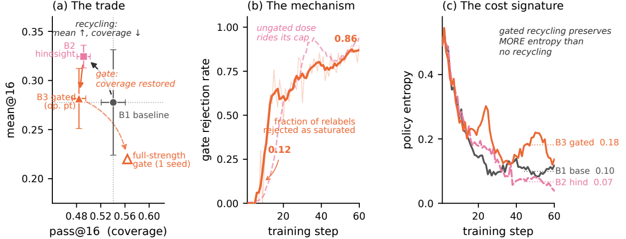
Figure 7: Recycling-induced sharpening and its derived mitigation (Countdown, tier 1). (a) Three seeds, both axes: recycling (B2) buys mean@16 with pass@16 coverage; the utility gate (B3) restores coverage to baseline keeping \sim 60\% of the gain; full-strength gating (corrected decay, 1 seed) pushes coverage above baseline at the cost of the mean — the gate threshold traces a mean-vs-coverage frontier. (b) The mechanism in-run: the gate’s rejection rate rises monotonically as the model’s reachable set saturates its relabel destinations, while the ungated dose rides its cap. (c) Gated recycling preserves more policy entropy than no recycling — admitted relabels are a spread-preserving gradient.
