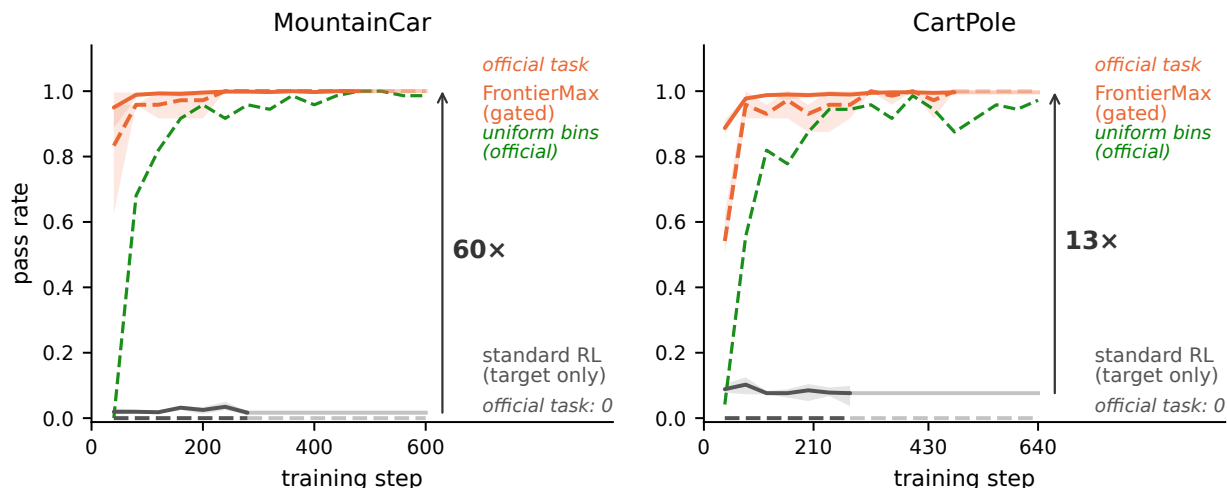
Figure 6: Gym control, trained to plateau (3 seeds, matched episodes) . Solid: mean pass rate across curriculum bins; dashed: the official task (MountainCar flag / CartPole survive-400). Standard RL flatlines at zero on the official task; a uniform-over-bins control (green) also cracks it — slower and off-ceiling — isolating what the teacher adds (speed, seed-stability) from what task spread adds (existence of the gradient); the gated FrontierMax stack converges to 1.000 \pm 0.000 .
