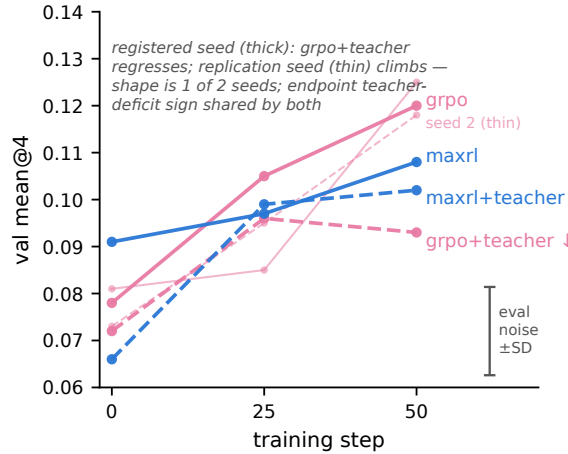
Figure 6: GSM8K 2 \times 2 , val mean@4 over training. Both GRPO seeds shown as paired trajectories (registered seed thick, replication thin); gray bar: repeated-eval noise floor of one fixed checkpoint ( \pm \text{SD } .0094 ), drawn once as a scale. On the registered run GRPO+teacher is the only cell that regresses in its second half; the replication seed climbs instead. §6.7 gives the statistics and the steering telemetry that separates the two seeds.
