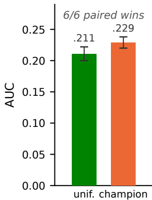
(c) Maze (3 seeds)
