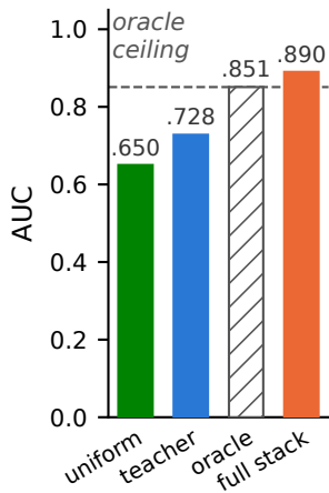
(a) Skill chain (5 seeds)
