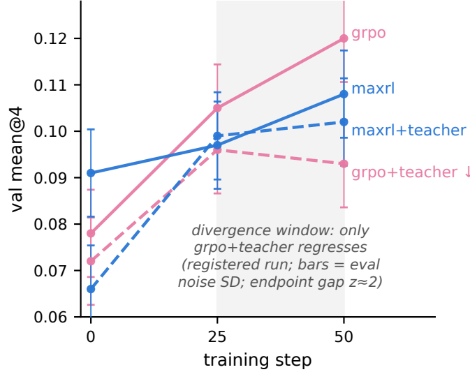
Figure 7: GSM8K 2×2 (pre-registered; registered run shown; error bars = measured same-model eval noise, SD .0094) . GRPO+teacher is the only cell that regresses in its second half (P-G2 on this run; the load-bearing statistic is the endpoint gap vs. plain GRPO, z \approx 2 — the second-half dip alone is within noise; a replication seed with weaker measured steering climbed instead — §6.7); under MaxRL the identical teacher trains stably to its best value but does not beat uniform at this budget (P-G1: null).
