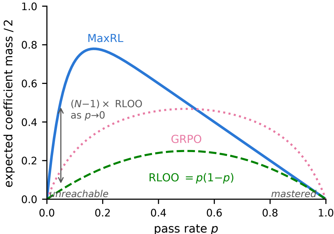
Figure 1: The estimator is the curriculum. Left: the derived utility u_N(p) = (1 - (1 - p)^N) - p — half the estimator’s expected coefficient mass A_N = 2u_N (Prop. 1) — for growing rollout budgets N . The peak p^* \approx \ln N/N walks toward harder prompts as compute grows; the utility vanishes exactly at p \in \{0, 1\} . Right: all three curves are exact expected half-mass at N=16 for the estimators as deployed (GRPO with sample-SD normalization: \sqrt{\frac{N-1}{N}} \frac{1}{N} \mathbb{E} \sqrt{K(N-K)} , K \sim \text{Bin}(N, p) ; MC-verified against the code). MaxRL concentrates \rightarrow (N-1) \times more mass than RLOO on frontier prompts (Prop. 2); in the mastered tail MaxRL and RLOO decay together at first order (both \rightarrow q = 1 - p ; MC artifact verify_guidance_math.json ) while GRPO’s variance normalization keeps \sim (N-1)/\sqrt{N} \times their relative mass there — the maintenance-of-easy-tasks its curriculum arms lose in §6. RLOO’s profile is exactly the published “learnability” objective — the N=2 slice.
