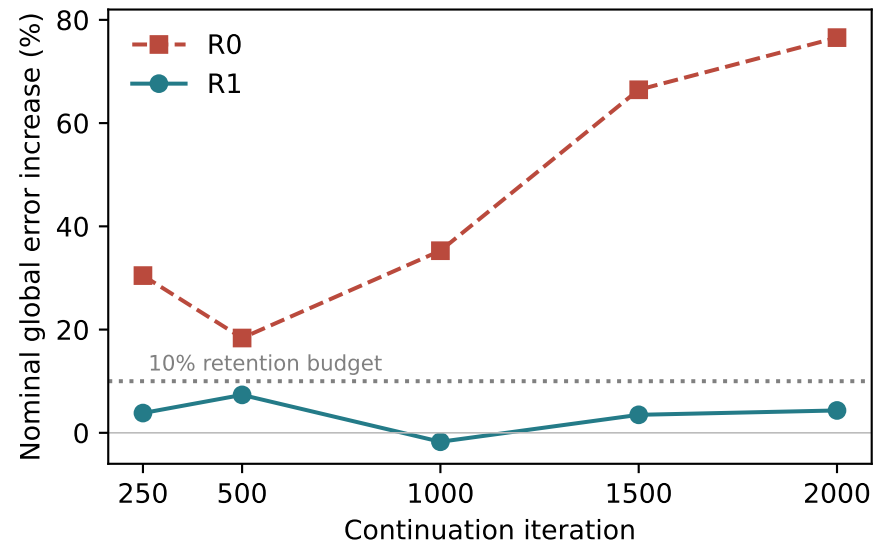
Seed 8600 continuation
