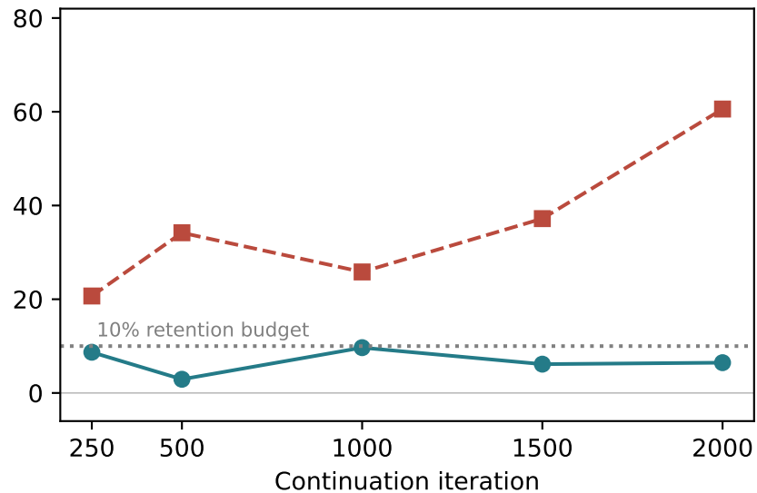
Seed 8601 continuation
