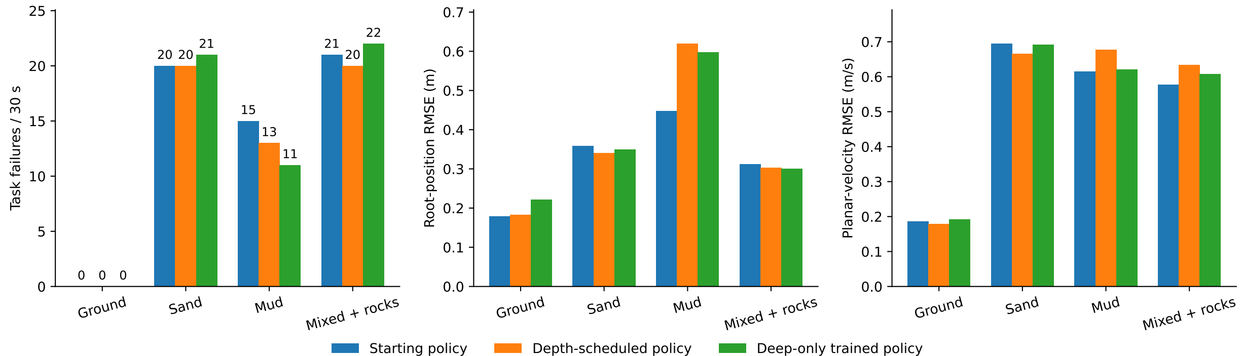
Completed-policy evaluation: original 14 cm soil and original motion timing
