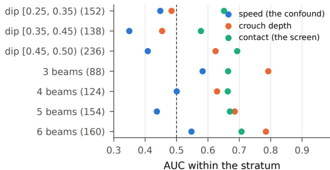
(b) Duck family: only the contact feature stays above chance everywhere
