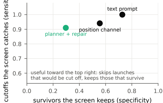
(c) As a filter at 0.20 s: usable for stepping, not for ducking
