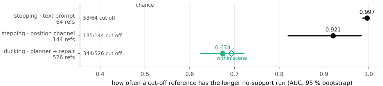
(a) One reference feature ranks the controller's cutoffs in three corpora
