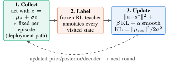
Fig. 2. One DAgger round ( \times 2,000 ). Rollouts are collected on the deployment (prior) path with episodic noise; a frozen explicit-command teacher labels visited states; the CVAE updates with action matching, a closed-form KL from the residual-to-prior posterior (tied \sigma ), and a latent smoothness term. The dashed return edge makes it DAgger rather than behavior cloning. At deployment: z_{\text{cmd}} = \mu_\rho (deterministic), no teacher, no posterior, no explicit reference to the actor.
