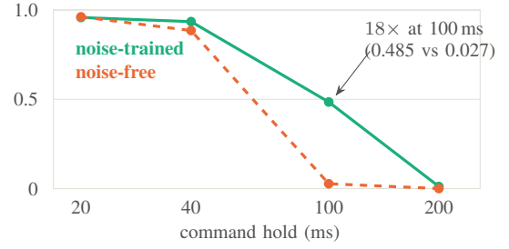
Fig. 3. Train-time latent noise buys command-latency robustness . Completion vs. zero-order hold on z_{\text{cmd}} (refresh every k ticks at 50 Hz; 1,024 rollouts per point, seed 404). The noise-trained code and the noise-free deterministic encoder are identical at nominal rate and diverge 18\times at 100 ms; both fail at 200 ms.
