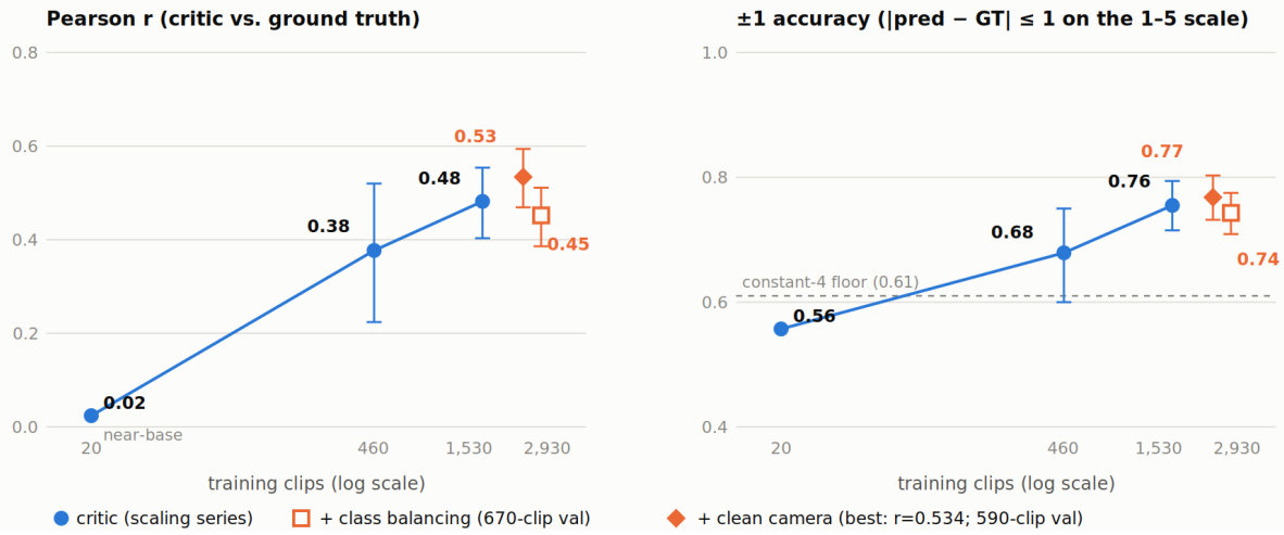
Fig. 2 — Critic quality vs. training data (scene-level holdout, 95% clip-bootstrap CIs)
