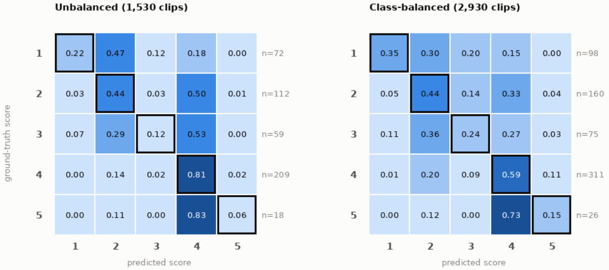
Fig. 5 — Class balancing shifts recall toward the rare scores (row-normalized; n per row at right)
