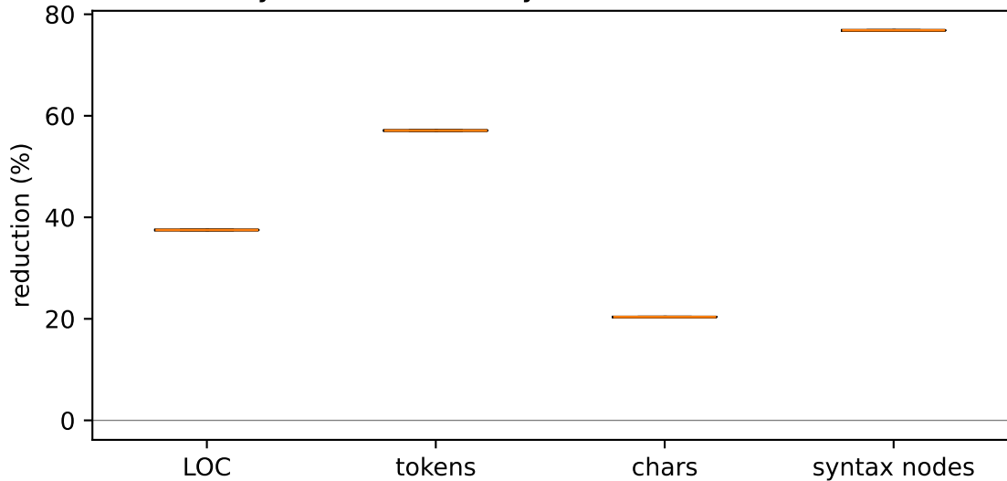
LD Python vs RDFLib Python — surface reduction
