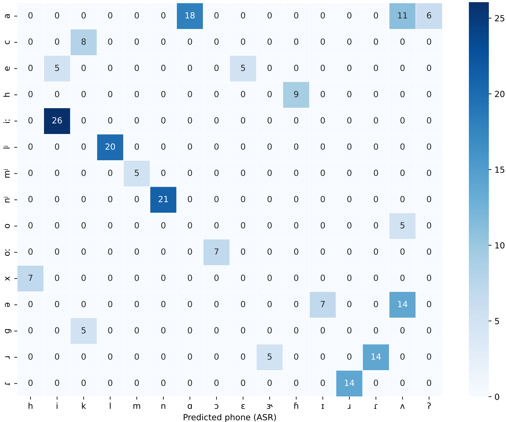
Diagnosis confusion — Ensemble (2-way, gibbs) (min freq=5)
