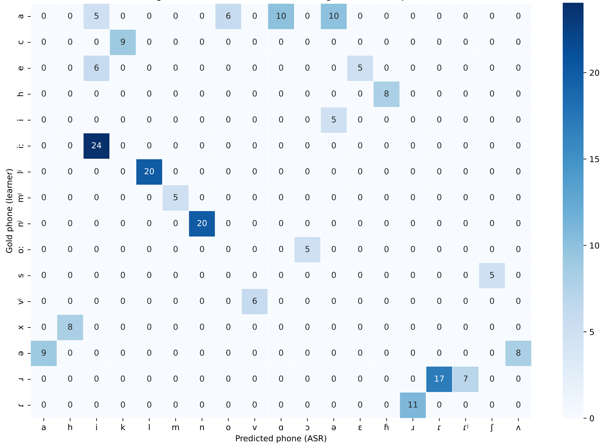
Diagnosis confusion — Ensemble (sel/gibbs) (min freq=5)
