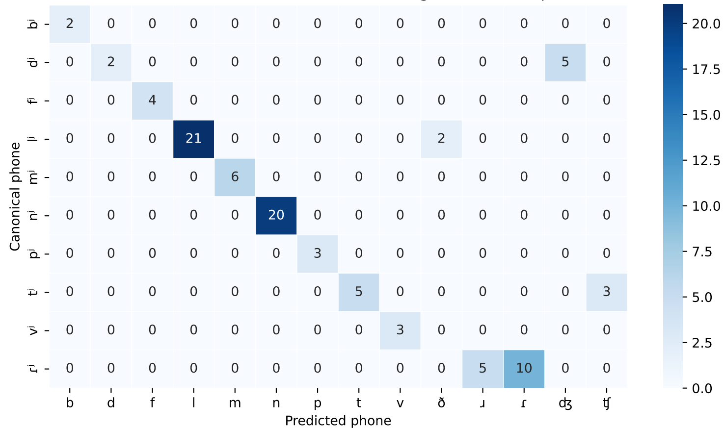
Substitution confusion — Ensemble (sel/gibbs) (min freq=2)
