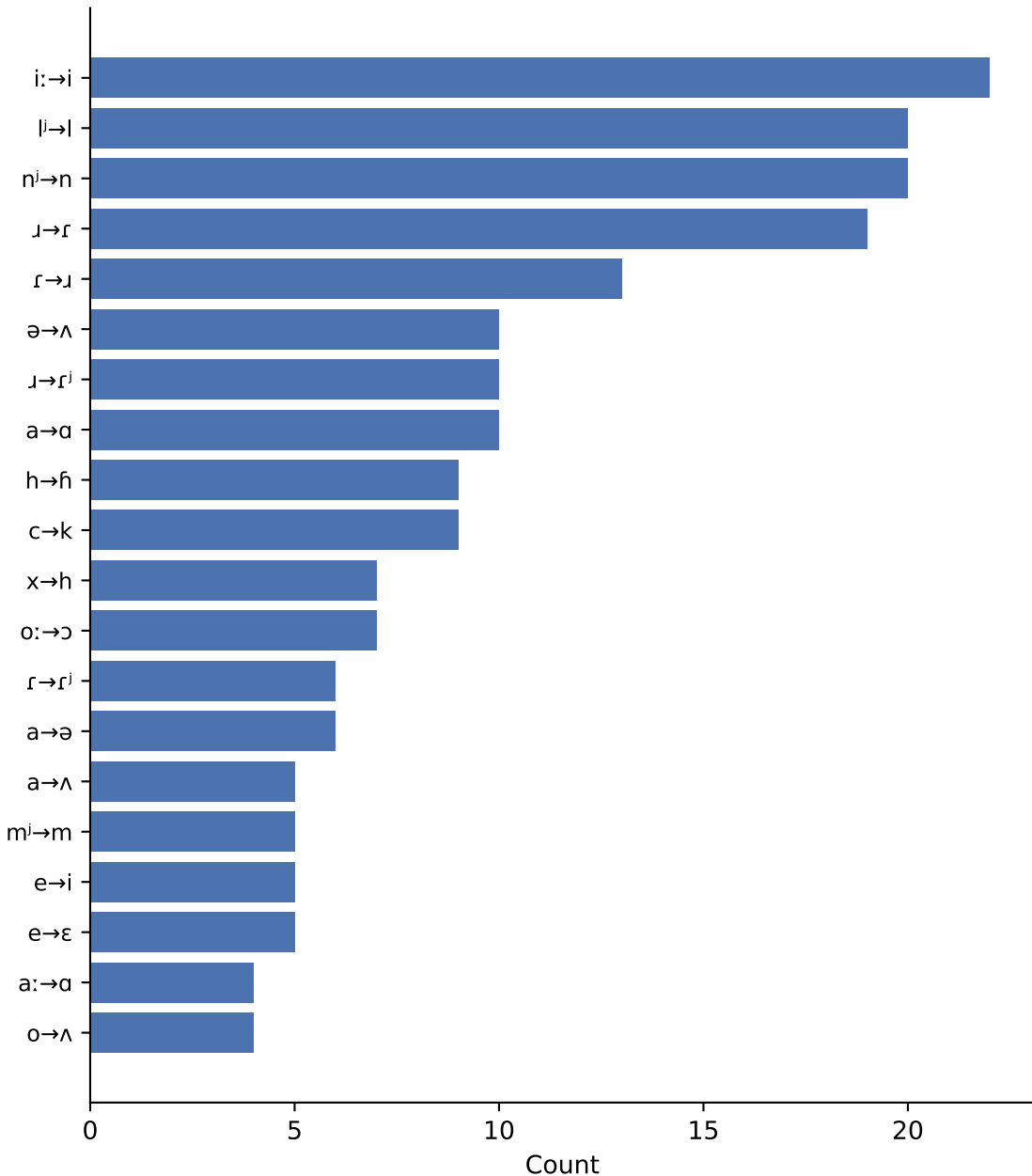
Top confusion pairs — Ensemble (2-way, sel/gibbs+pooled)
