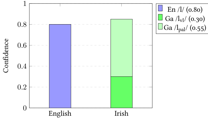
Figure 4.1: Phoneme pooling for a span with canonical /l/. Without pooling, the Irish model’s split distribution would give it lower confidence than English and lose. Summing probability mass across the broad/slender family (shaded, 0.85 total) beats English (0.80), and the Irish model’s top prediction /l/ is selected.
