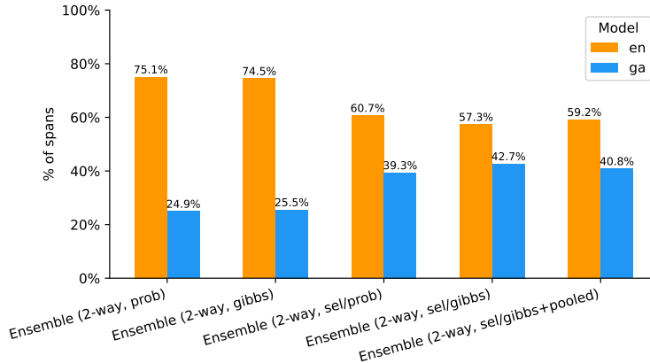
Figure 6.1: Ensemble winner contributions, en/ga
