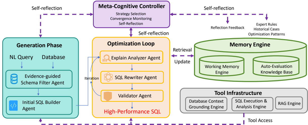
Fig. 2: Overview of OPTSQL
