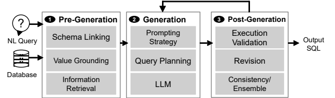
Fig. 1: Overview of a typical Text-to-SQL pipeline, illustrating the Pre-Generation, Generation, and Post-Generation stages
