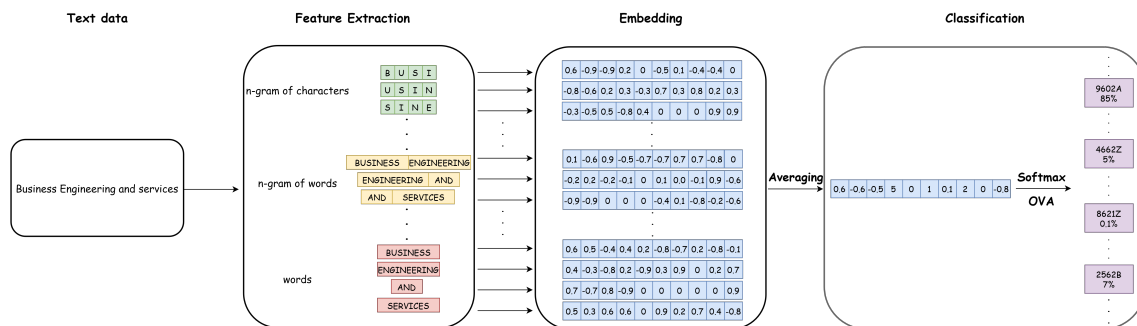
Figure 1: Diagram of FastText architecture
