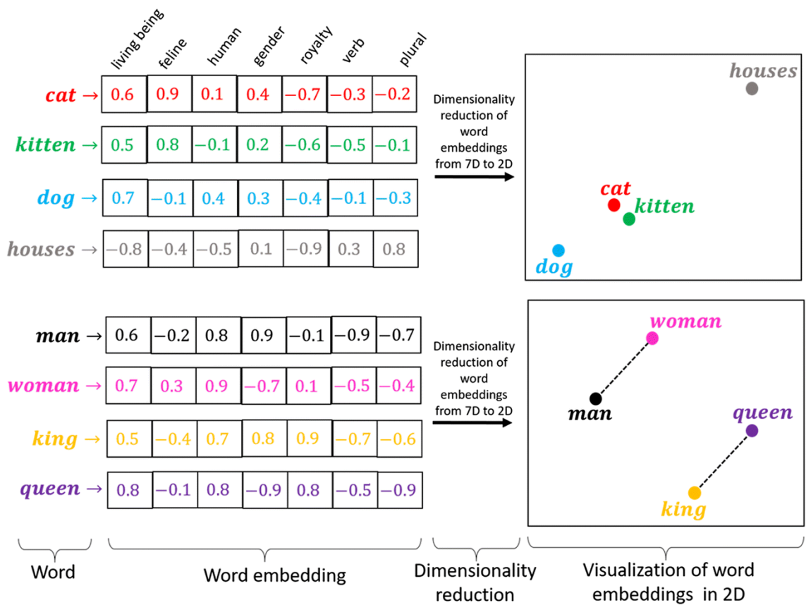
Figure 2: Illustration of lexical embedding. Source: Blog post Word Embedding: Basics
