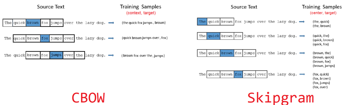
Figure 4: Illustration of the difference between CBOW and Skip-gram approaches
