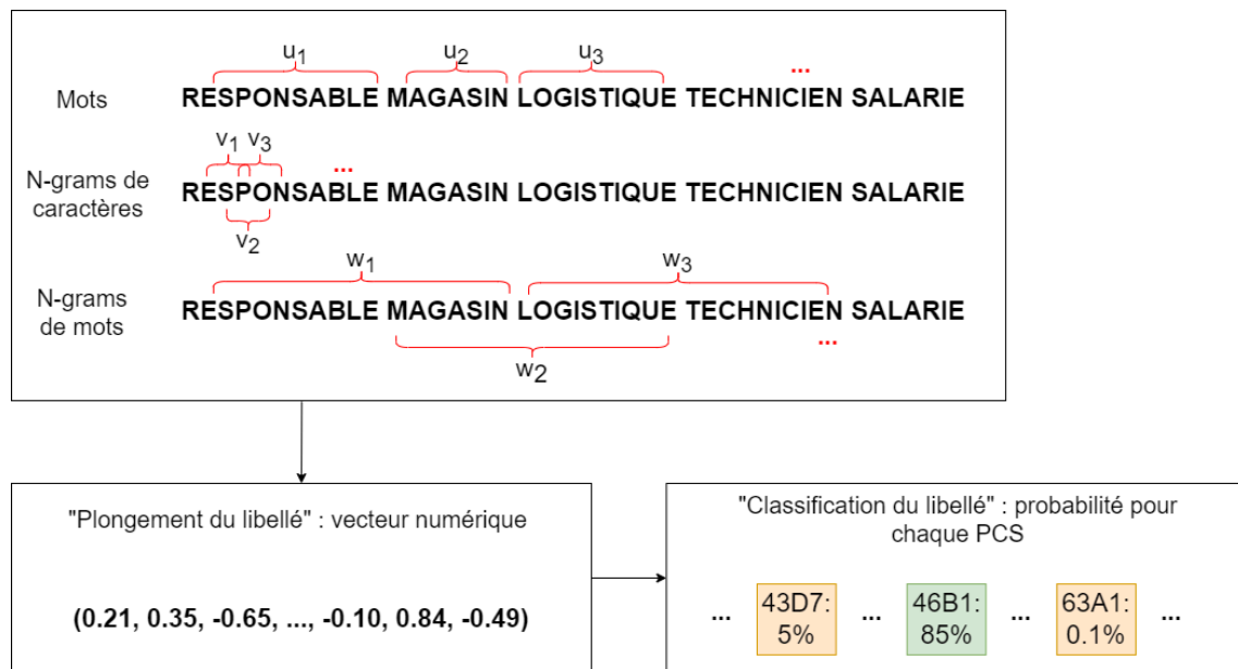
Figure 5: Illustration of the fastText model
