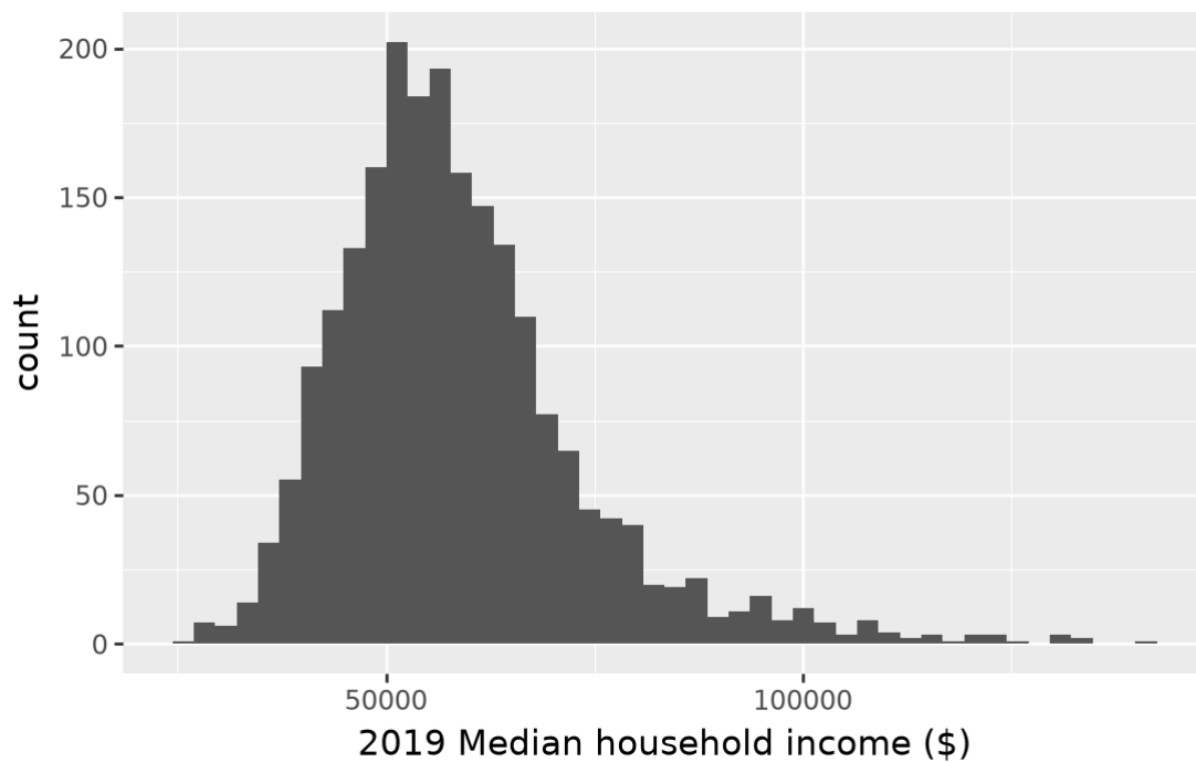
Figure 5. – Question 2, avant normalisation
